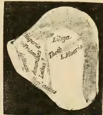
FIG. 7.—SKETCH OF MARS AS IT APPEARED ON MAY 21ST, 1886. (AFTER PERROTIN.)
